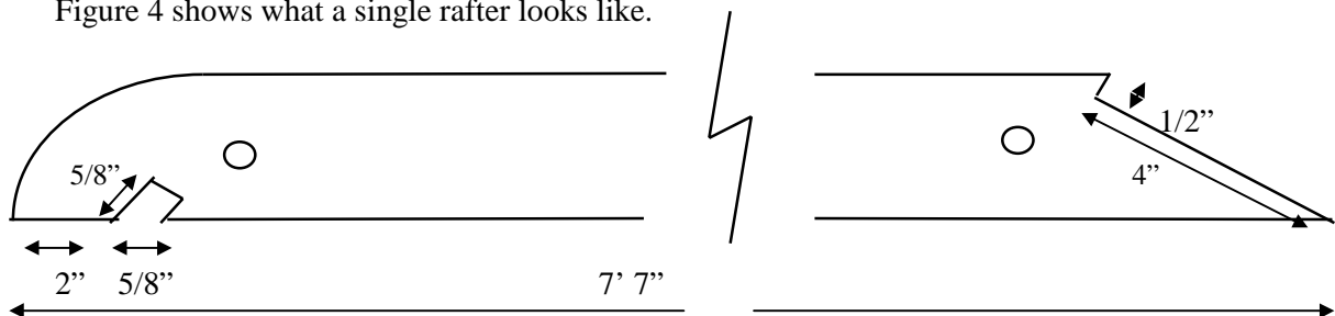
Figure 4: Rafter layout.
