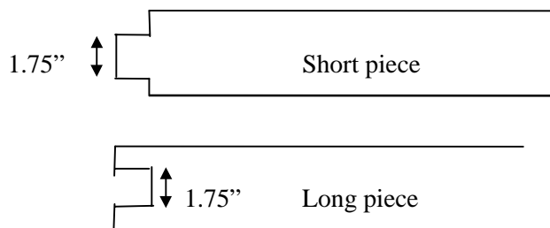
Figure 3: Notches for door frame.
